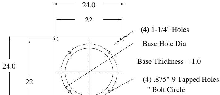
FOUNDATION PLATE
