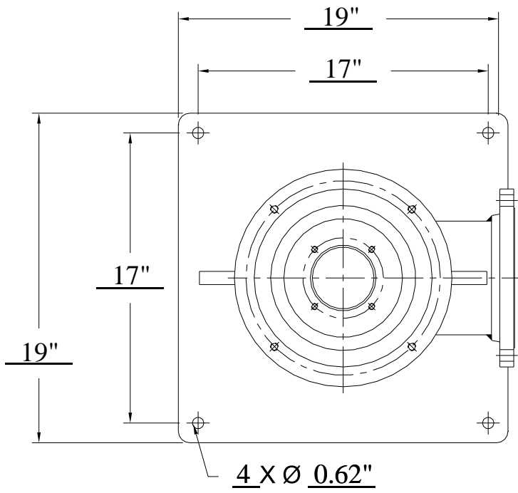
SQUARE BASE
